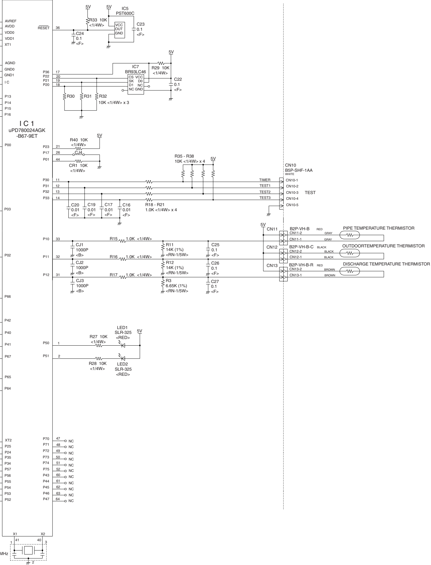
CONTROLLER PCB ASSEMBLY ( MAIN PCB ) K01DI-0400HUE-C1
