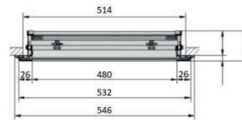
Return air diffuser
