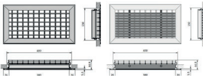
Wall mounted diffuser
