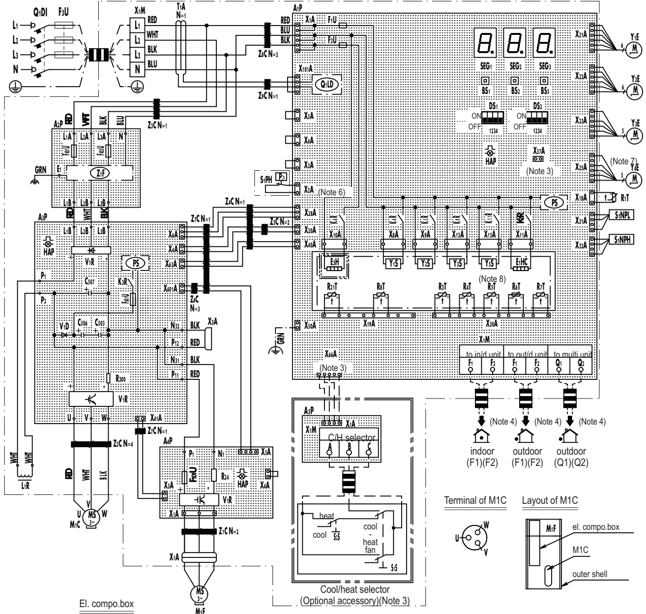
Wiring diagram
