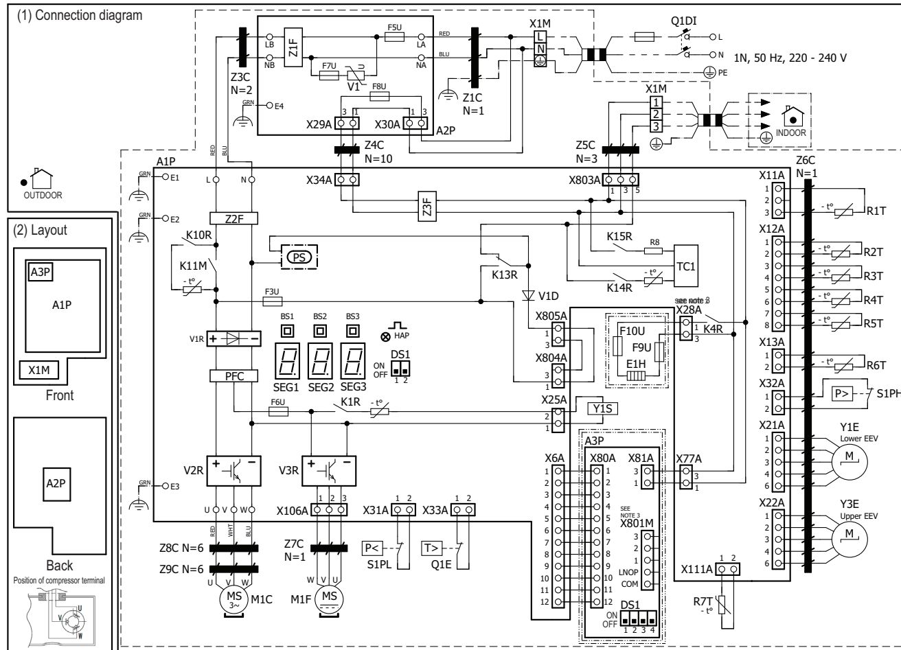
(1) Connection diagram
