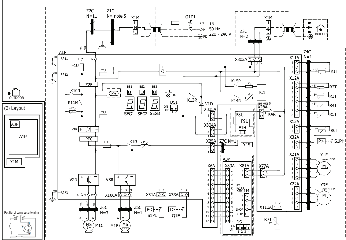
(1) Connection diagram
