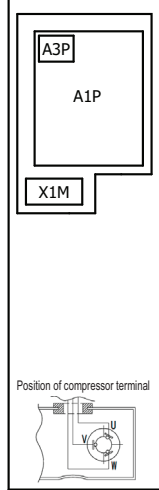
(2) Layout
