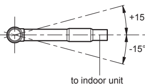
Triple connection type ( Gas )
