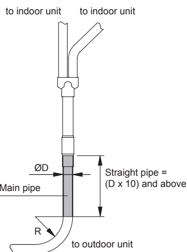
Twin connection type
