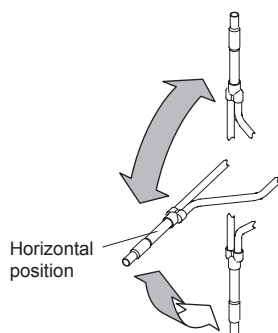
Twin connection type
