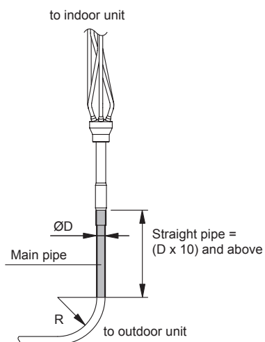
Triple connection type ( Liquid )
