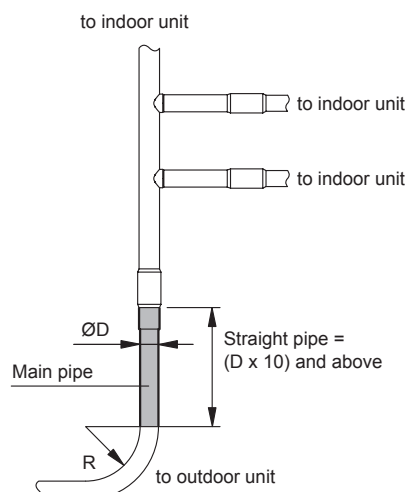
Triple connection type ( Gas )
