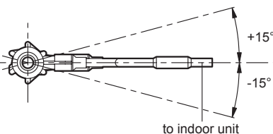
Triple connection type ( Liquid )
