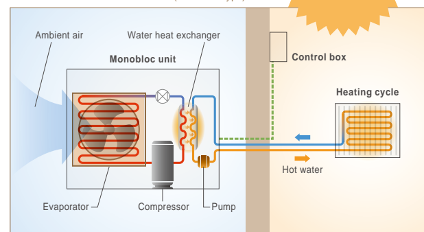
WATERSTAGE outline (Monobloc type)
